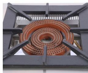
BULK COOKING BURNERS
